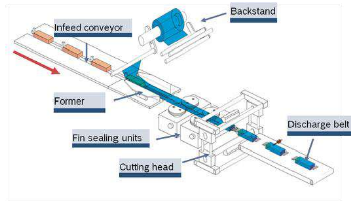
Figure 41: flow wrapping (Bosch packaging brochure)
